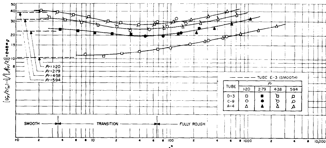
FIG. 13. Correlation of experimental results, using the heat-transfer similarity law.
