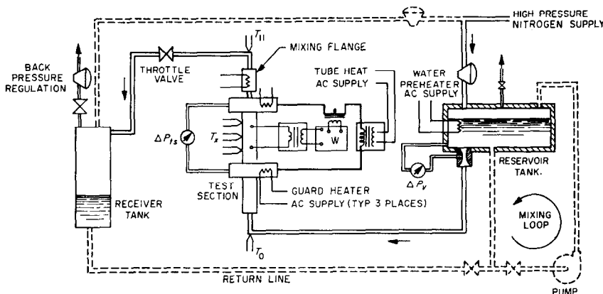
FIG. 1. Simplified test facility schematic.
