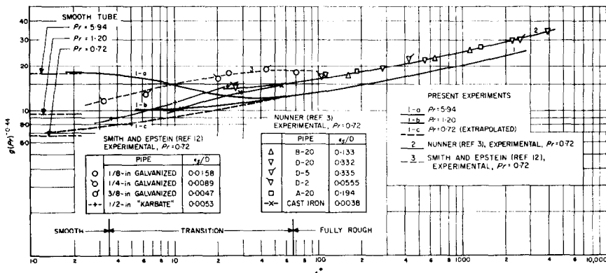
FIG. 15. Comparisons—rough tube heat-transfer experimental results.
