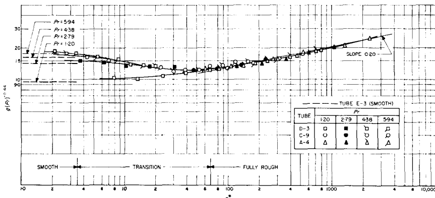
FIG. 14. Correlation of experimental results, using the heat-transfer similarity law and a power law for Prandtl number.
