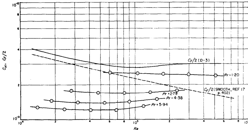
FIG. 6. Heat-transfer coefficient vs. Reynolds number for tube D-3 ( \epsilon_s/D = 0.0024 ) at Prandtl numbers 1.20, 2.79, 4.38 and 5.94.
