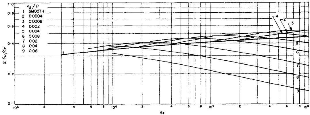
FIG. 19. Comparisons of heat-transfer to friction coefficient ratio vs. Reynolds number for Pr = 6.0 , generated from the similarity functions g[\epsilon^*; Pr] and A[\epsilon^*] .
