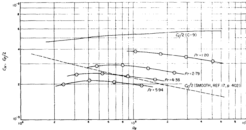
FIG. 7. Heat-transfer coefficient vs. Reynolds number for tube C-9 ( \epsilon_s/D = 0.0138 ) at Prandtl numbers 1.20, 2.79, 4.38 and 5.94.
