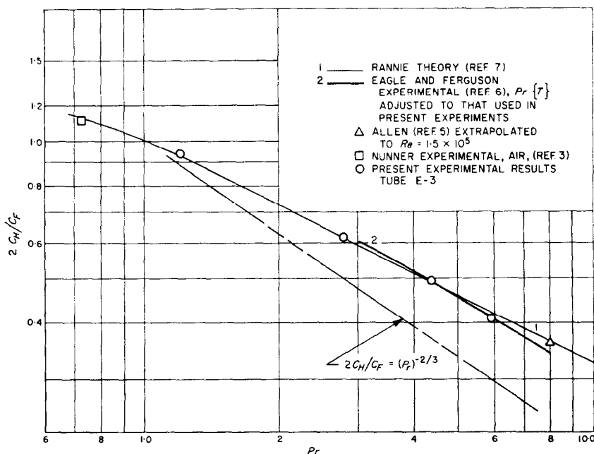
FIG. 5. Comparisons—Prandtl number influence on heat-transfer coefficients in smooth tubes at Re = 1.5 \times 10^5 .
