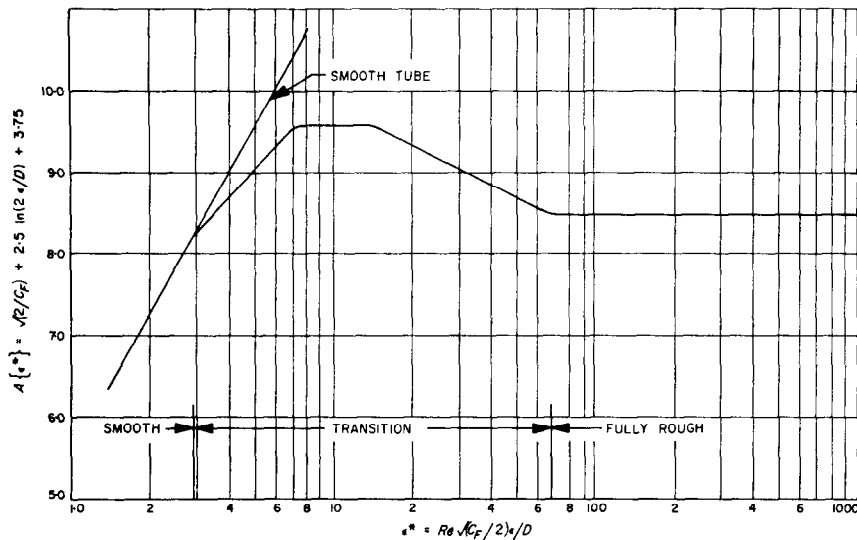
FIG. 12. Friction similarity function for close-packed sand-grain roughness.
