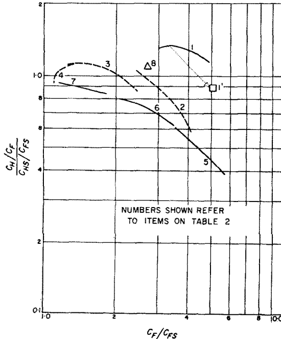
FIG. 16. Comparisons of experimental heat-transfer results for rough surface in relation to smooth surfaces.
