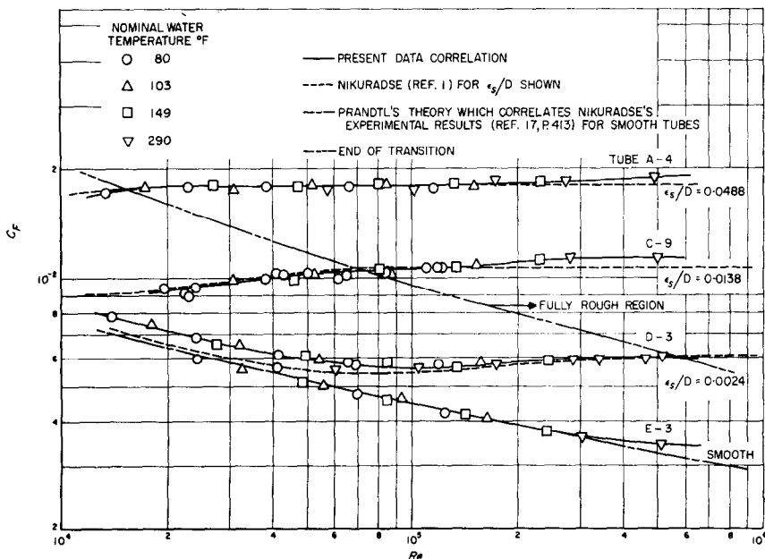
FIG. 4. Friction coefficient vs. Reynolds number for tubes E-3, D-3, C-9 and A-4.
