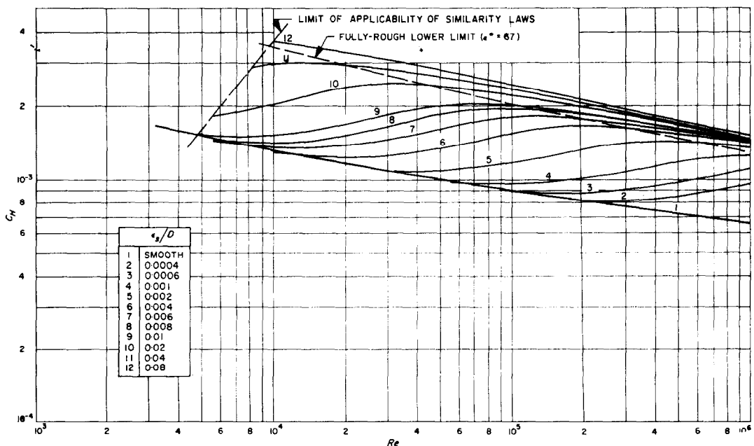
FIG. 18. Heat-transfer coefficient vs. Reynolds number for Pr = 6.0 , generated from the similarity functions g\{\epsilon^*; Pr\} and A\{\epsilon^*\} .
