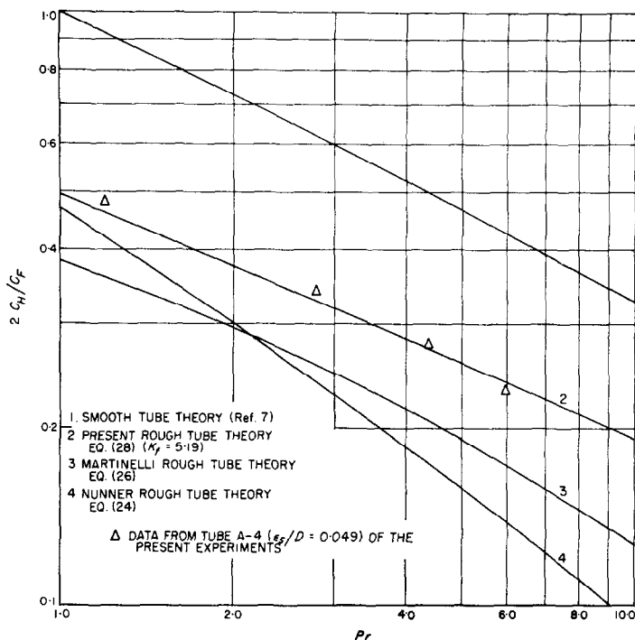
FIG. 17. Comparison of rough tube theories at Re = 1.5 \times 10^5 and \epsilon_s/D = 0.049 ( C_{FPR} = 0.018 ).
