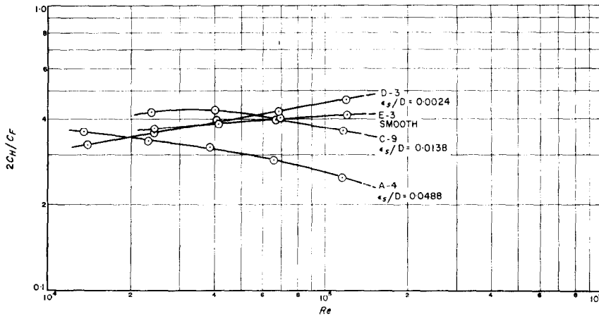
FIG. 11. Comparisons of heat-transfer and friction coefficients vs. Reynolds number for Pr = 5.94 .
