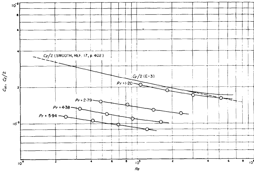
FIG. 9. Heat-transfer coefficient vs. Reynolds number for tube E-3 (Smooth) at Prandtl numbers of 1.20, 2.79, 4.38 and 5.94.
